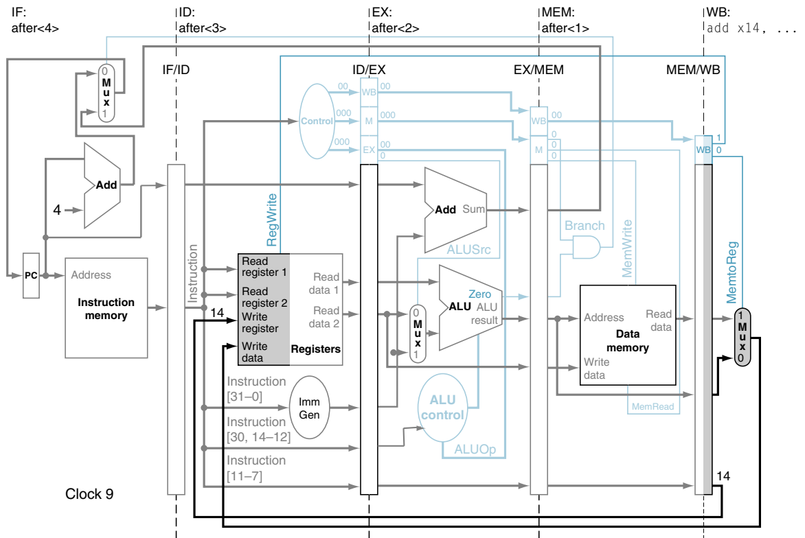
FIGURE e4.14.15 Clock cycle 9. The WB stage writes the ALU result in MEM/WB into register \times 14 , completing add and the five-instruction sequence. The instructions after add are shown as inactive for pedagogical reasons.
