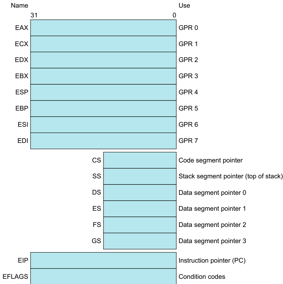
FIGURE 2.34 The 80386 register set. Starting with the 80386, the top eight registers were extended to 32 bits and could also be used as general-purpose registers.
