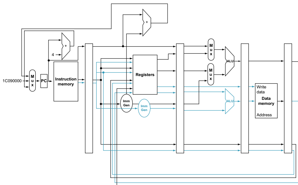
FIGURE 4.70 A static two-issue datapath. The additions needed for double issue are highlighted: another 32 bits from instruction memory, two more read ports and one more write port on the register file, and another ALU. Assume the bottom ALU handles address calculations for data transfers and the top ALU handles everything else.
